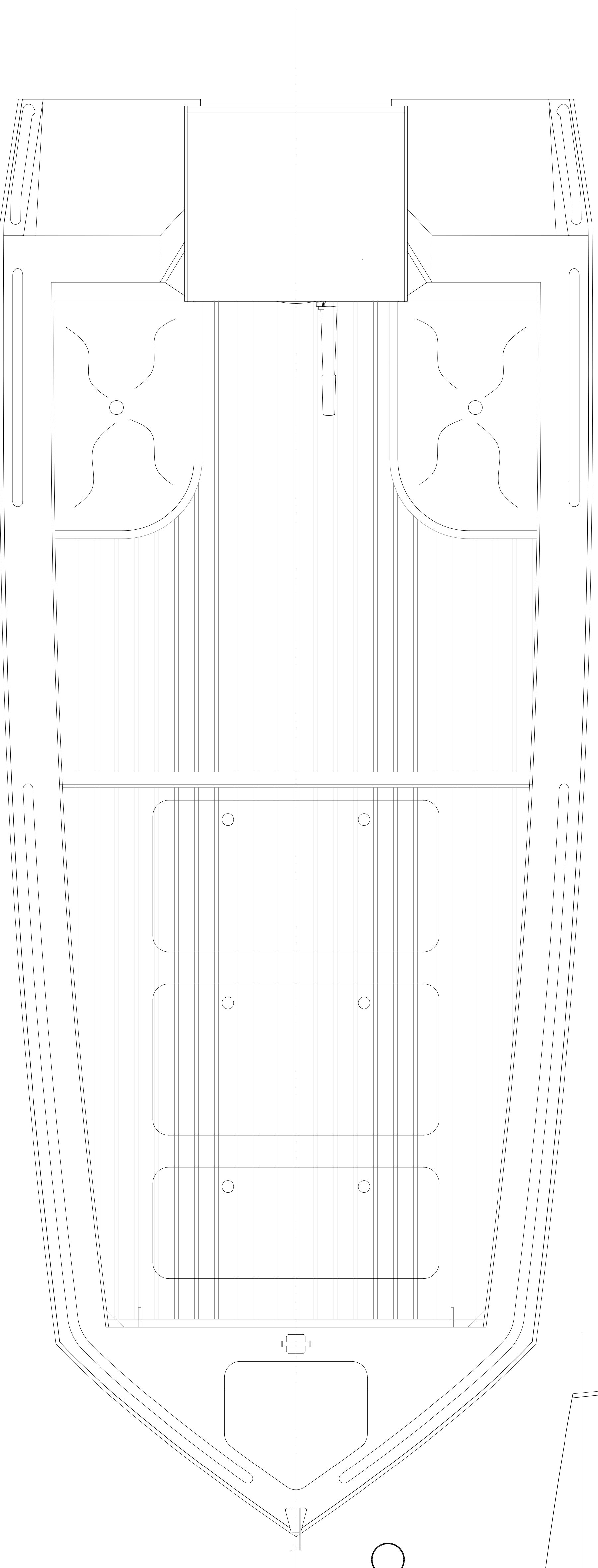
SECTION VIEW
